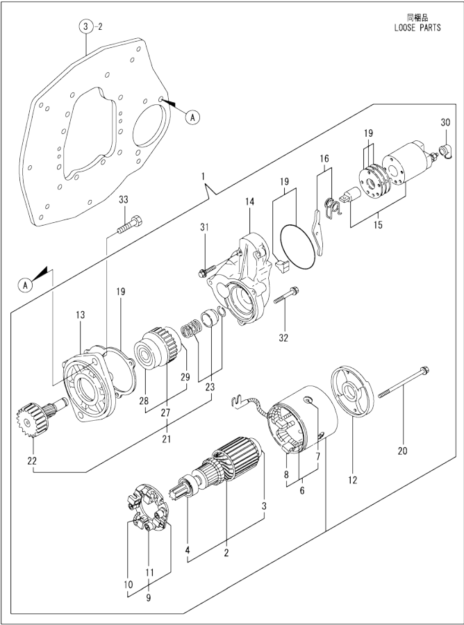
0CW10-M33100 3TNV84T-BGKL Fig.17. STARTING MOTOR
